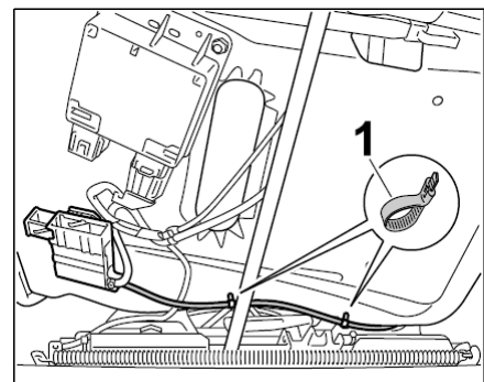
Securing wire harness at the seat frame
