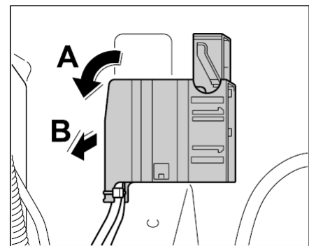
Removing airbag connector socket
